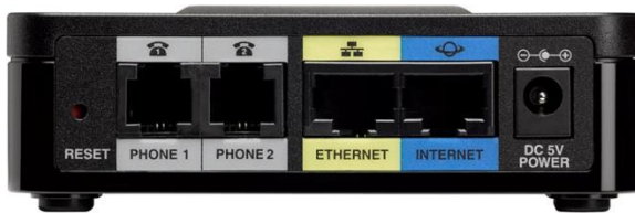
Figure 2. Ports on Cisco SPA122 ATA with Router
